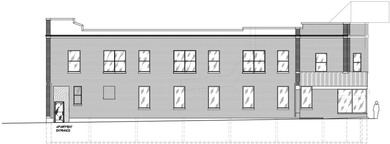
DAWSON AVE. NORTH WEST ELEVATION
