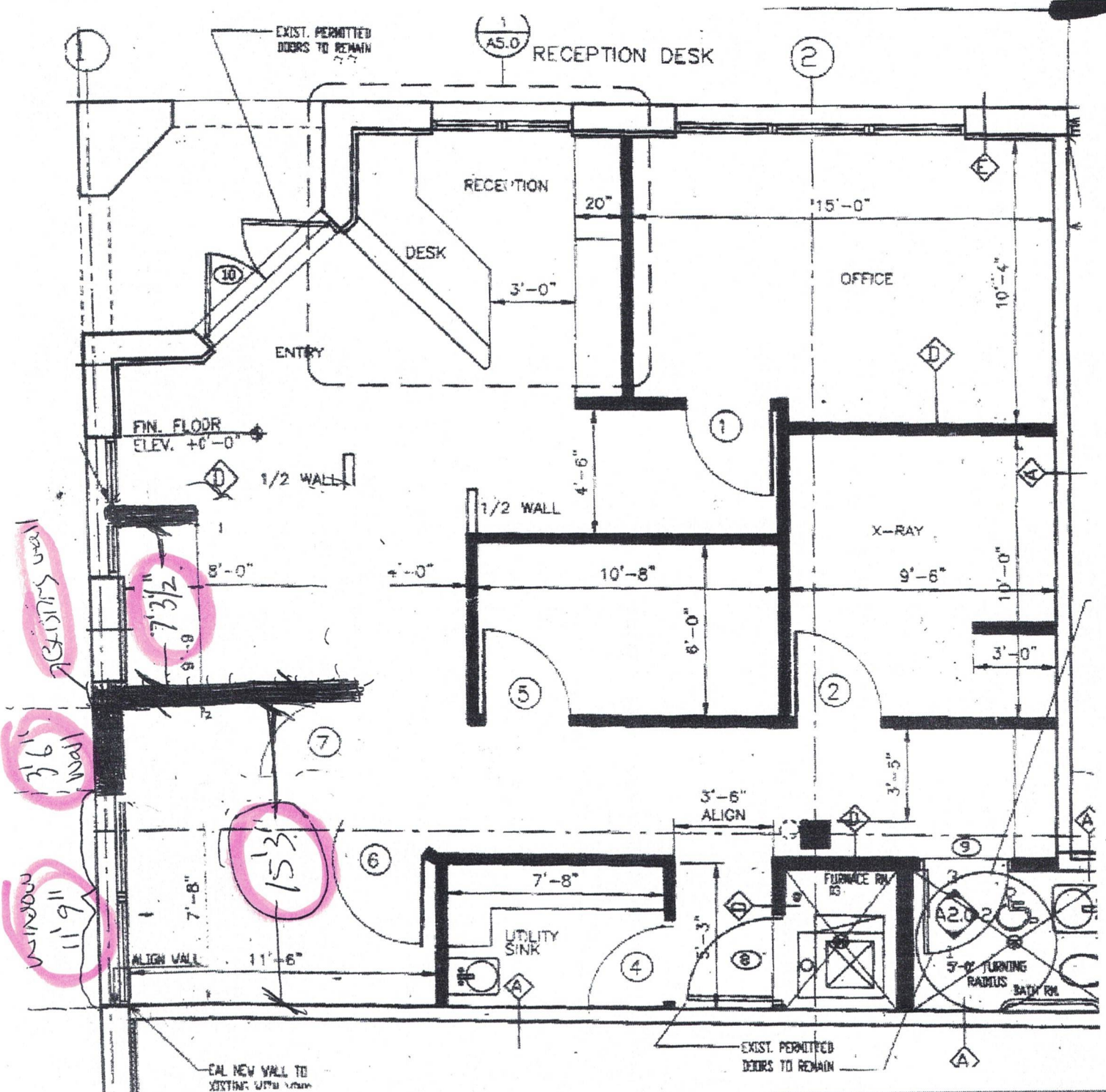
Floor Plan
