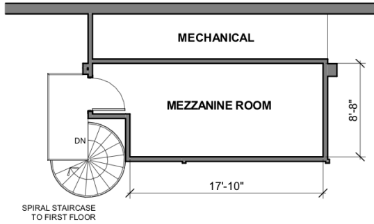
MEZZANINE 200 SF
