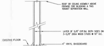
5 A1-3 WALL DETAIL # 4 NOT TO SCALE
