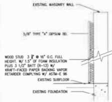
4 A1-3 WALL DETAIL # 1 NOT TO SCALE
