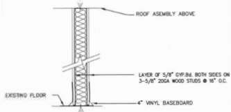
6 A1-3 WALL DETAIL # 5 NOT TO SCALE
