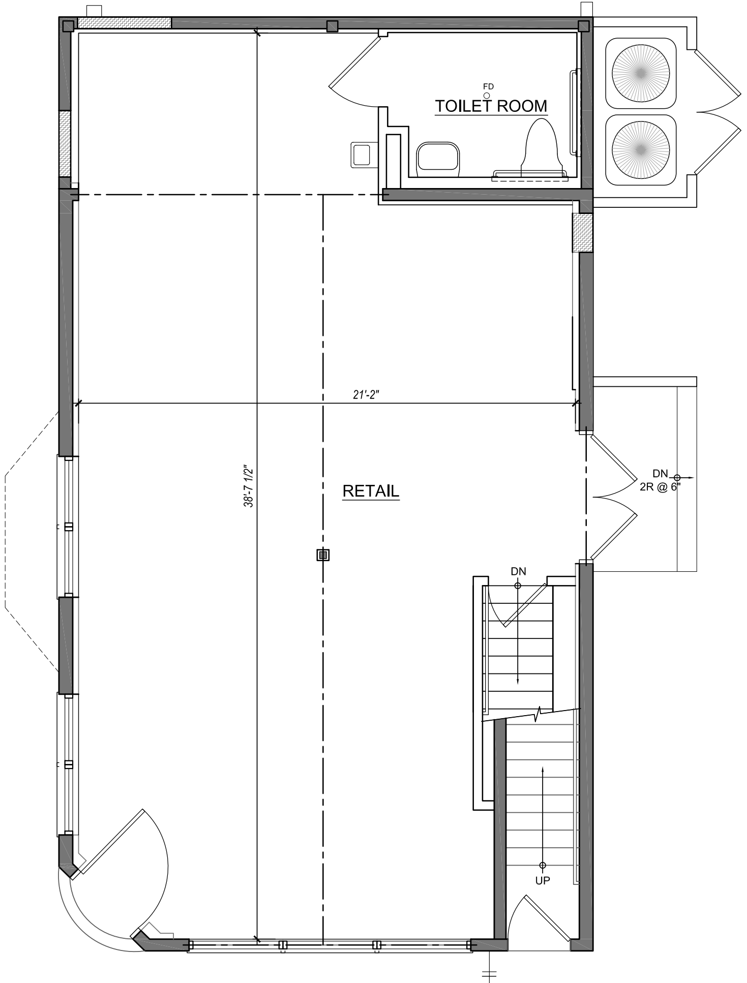
2 FIRST FLOOR PLAN 1/4"=1'-0"
